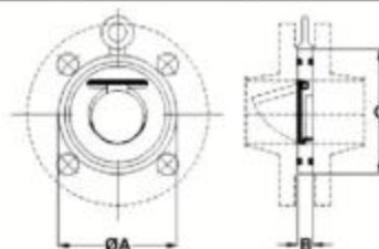
SINGLE PLATE CHECK VALVES
