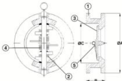
DUAL PLATE CHECK VALVES
